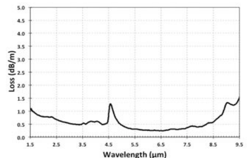
Typical Spectral Attenuation
