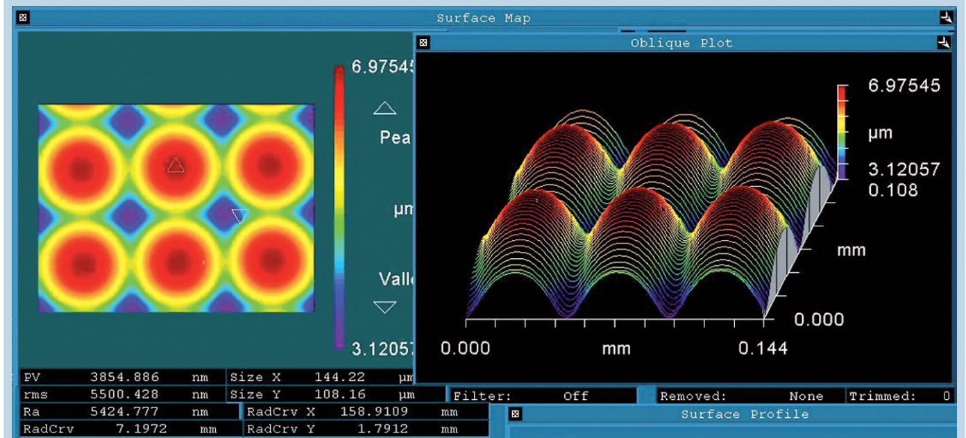
Microlens array surface profile
