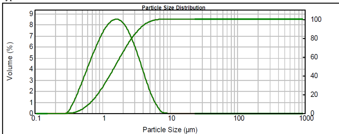
Typical PSD
