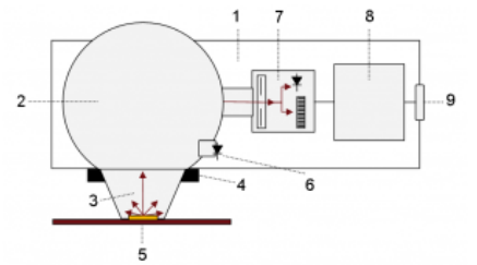
BTS256-LED for measurement of the luminous flux, spectrum, color, and color rendering index of single LEDs
