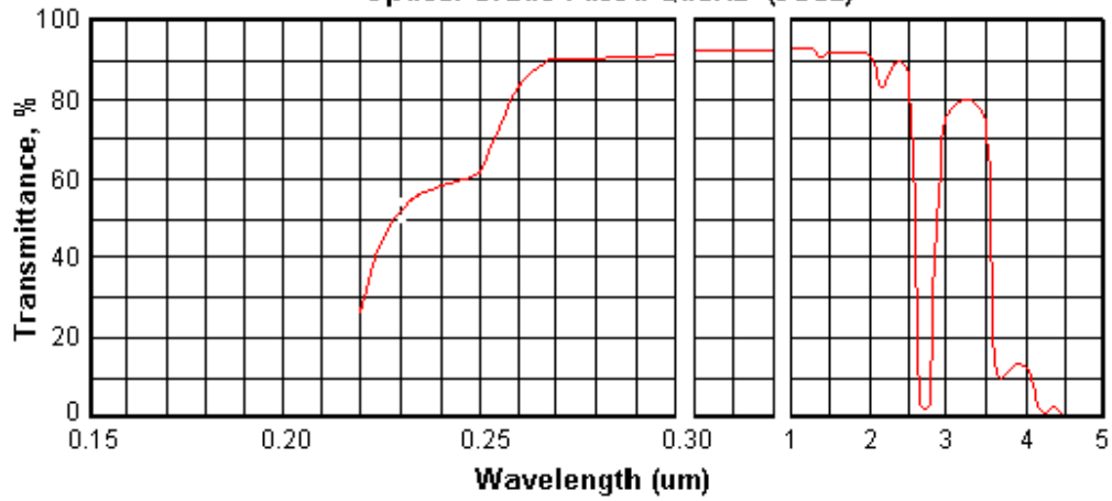
Full Spectrum Fused Silica (JGS3)
