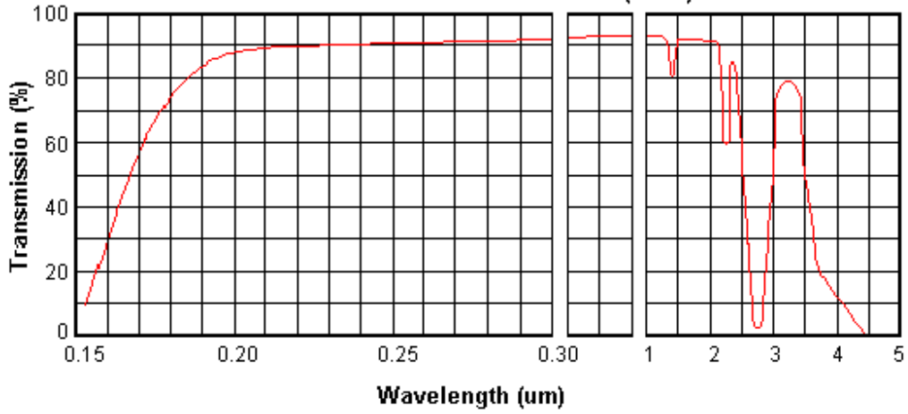
Optical Grade Fused Quartz (JGS2)
